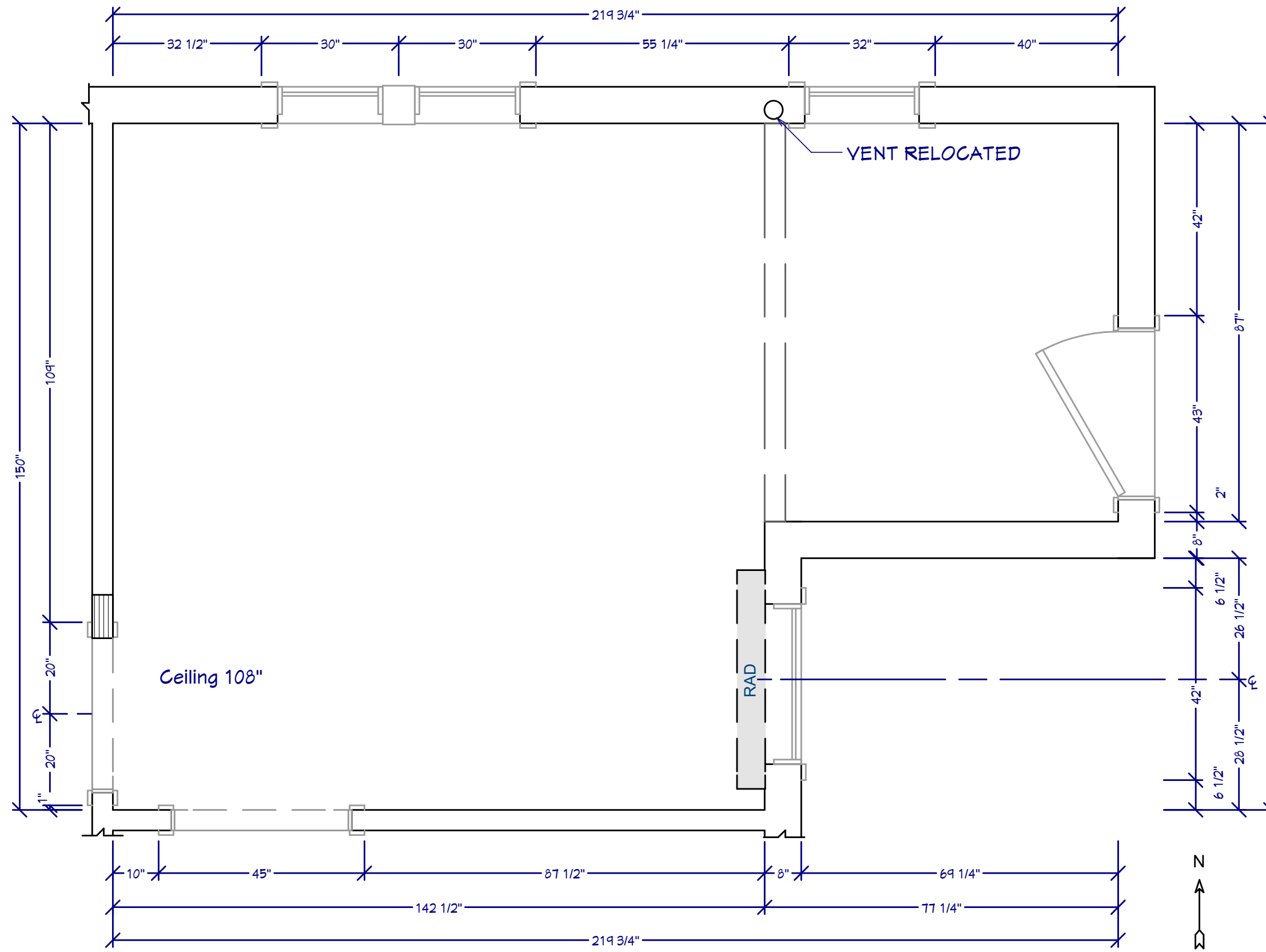
CONSTRUCTION PLAN 1/2" = 1'
