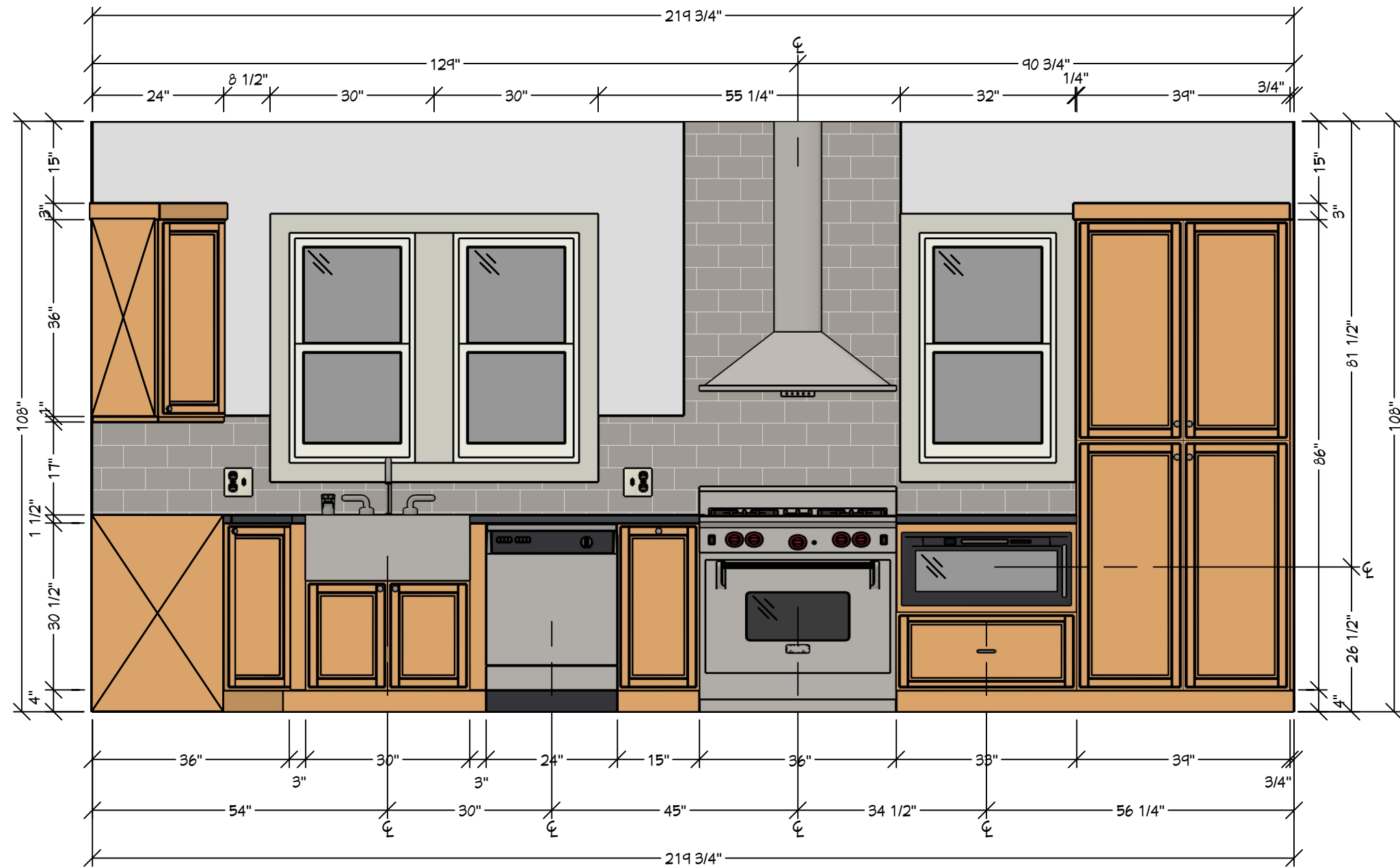
A MAIN WALL ELEVATION 1/2" = 1'
