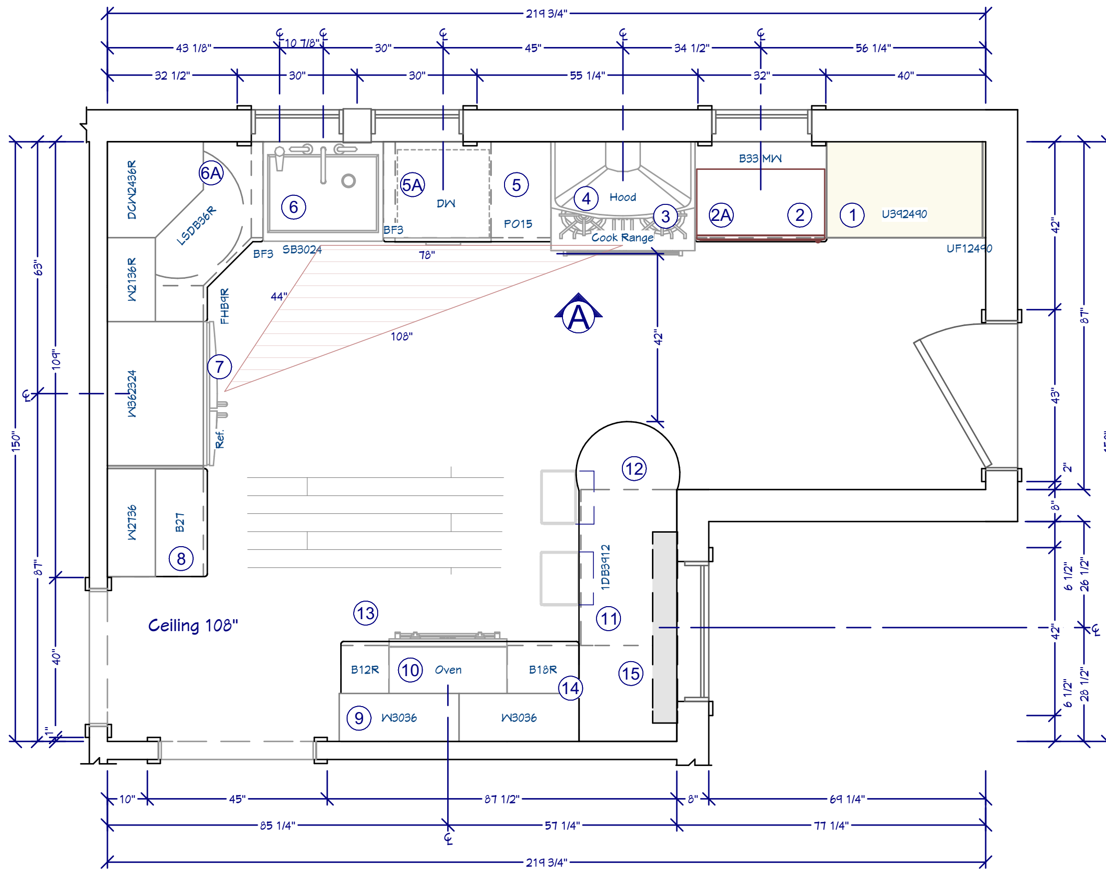
FLOOR PLAN 1/2" = 1'
