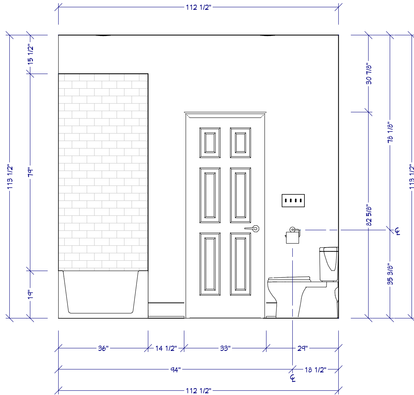
D ELEVATION D 1/2" = 1'
