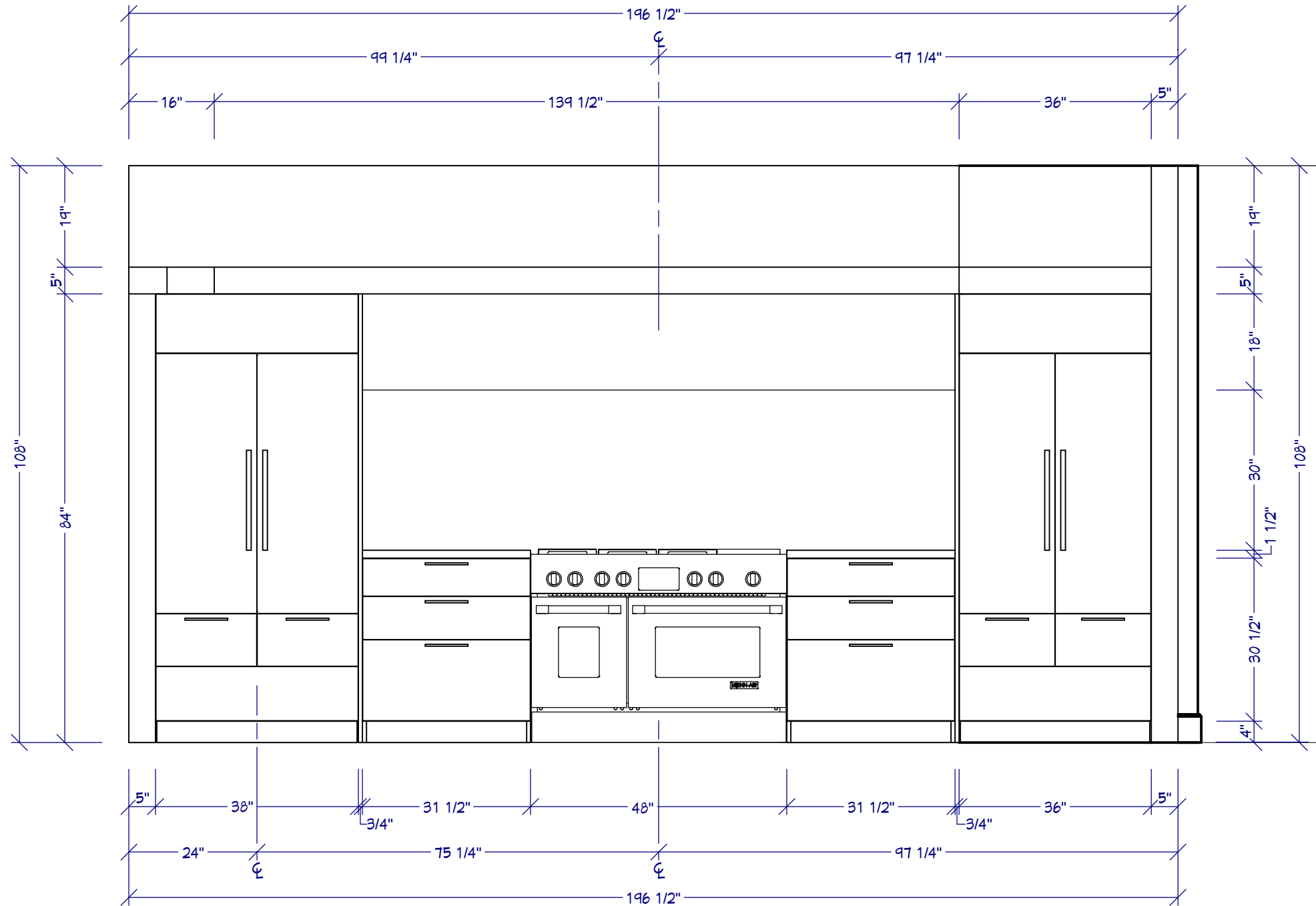
ELEVATION A 1/2" = 1'
