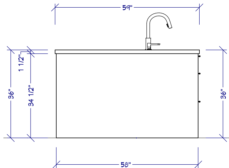
C ELEVATION C 1/2" = 1'
