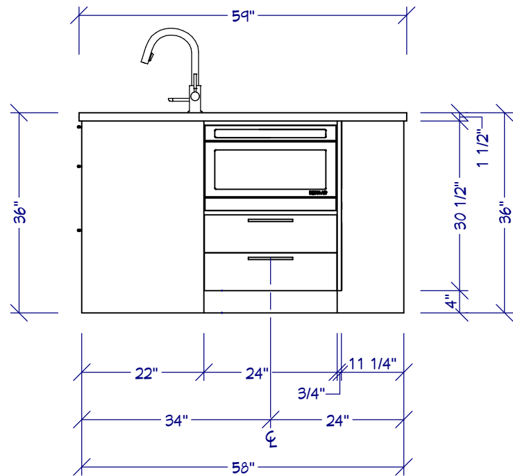
C ELEVATION C 1/2" = 1'
