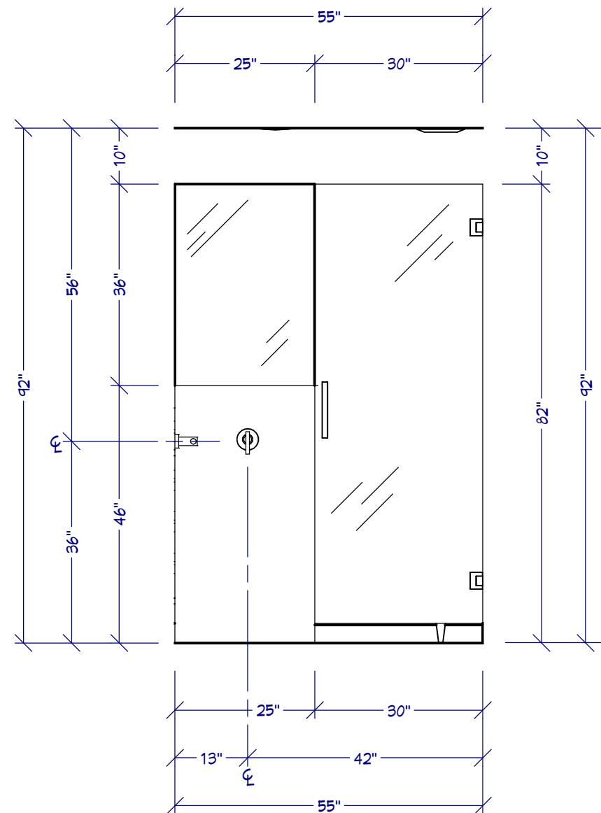
G ELEVATION G 1/2" = 1'
