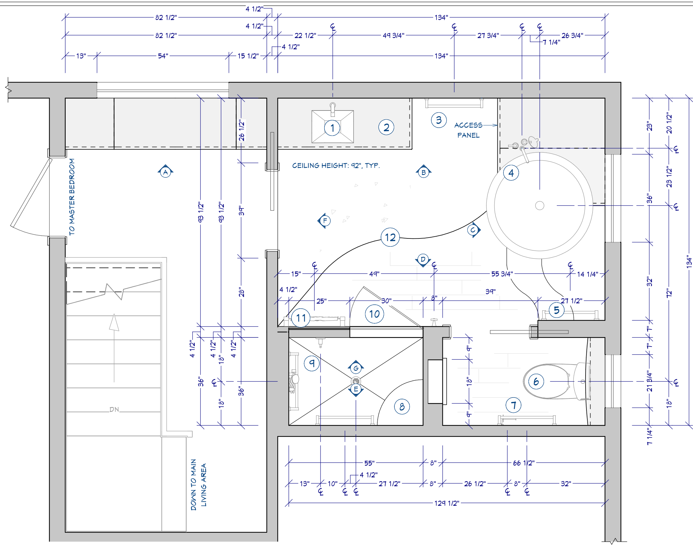
FLOOR PLAN 1/2" = 1'
