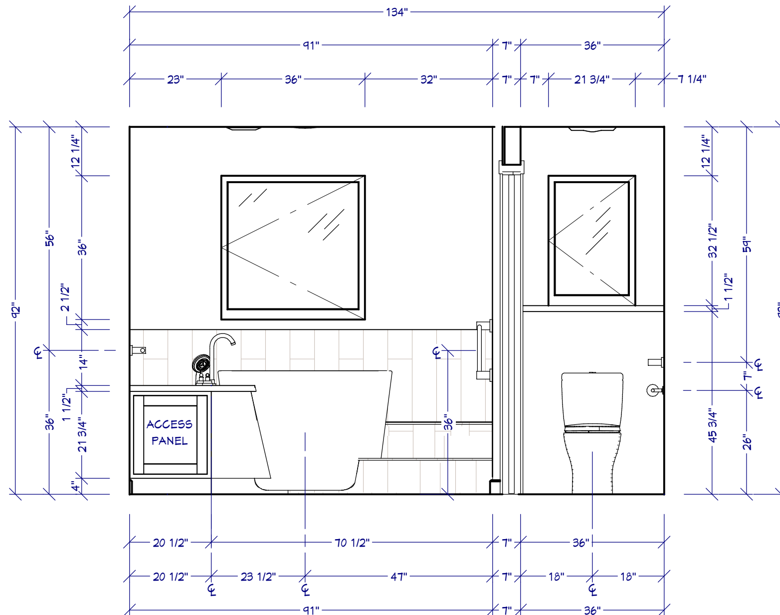
ELEVATION C 1/2" = 1'
