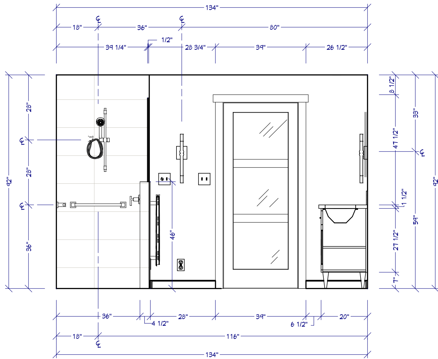
F ELEVATION F 1/2" = 1'
