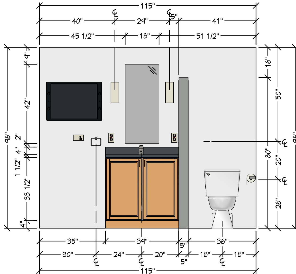
A MAIN WALL ELEVATION 1/2" = 1'
